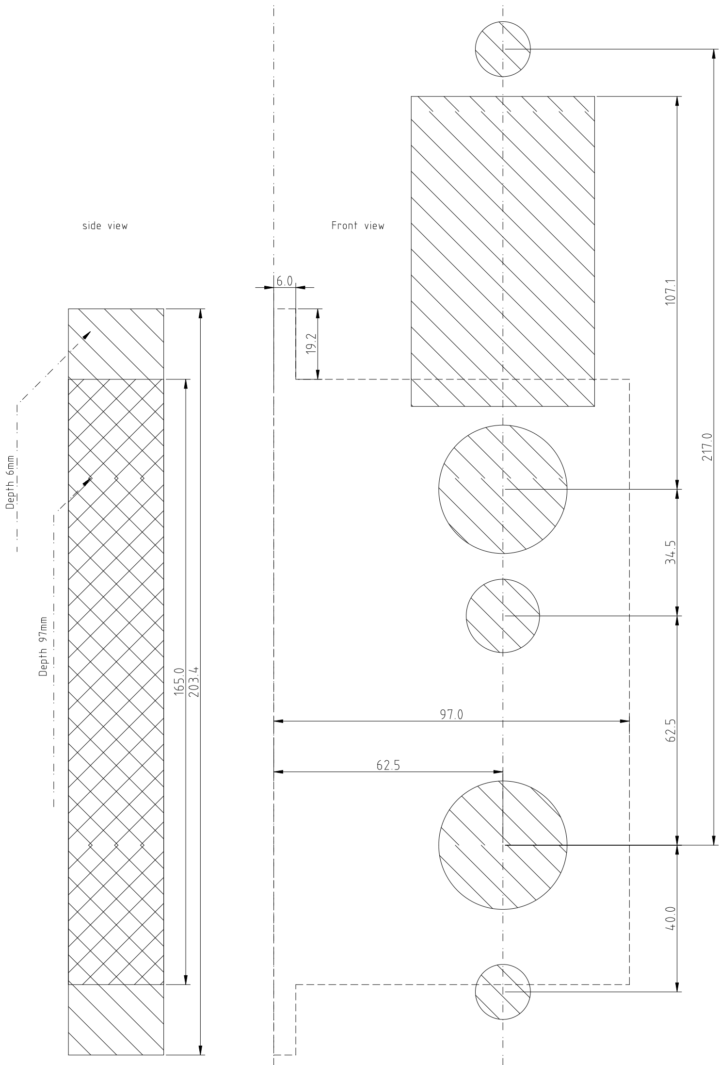
JCH2020 1:1 A3 Open holes
